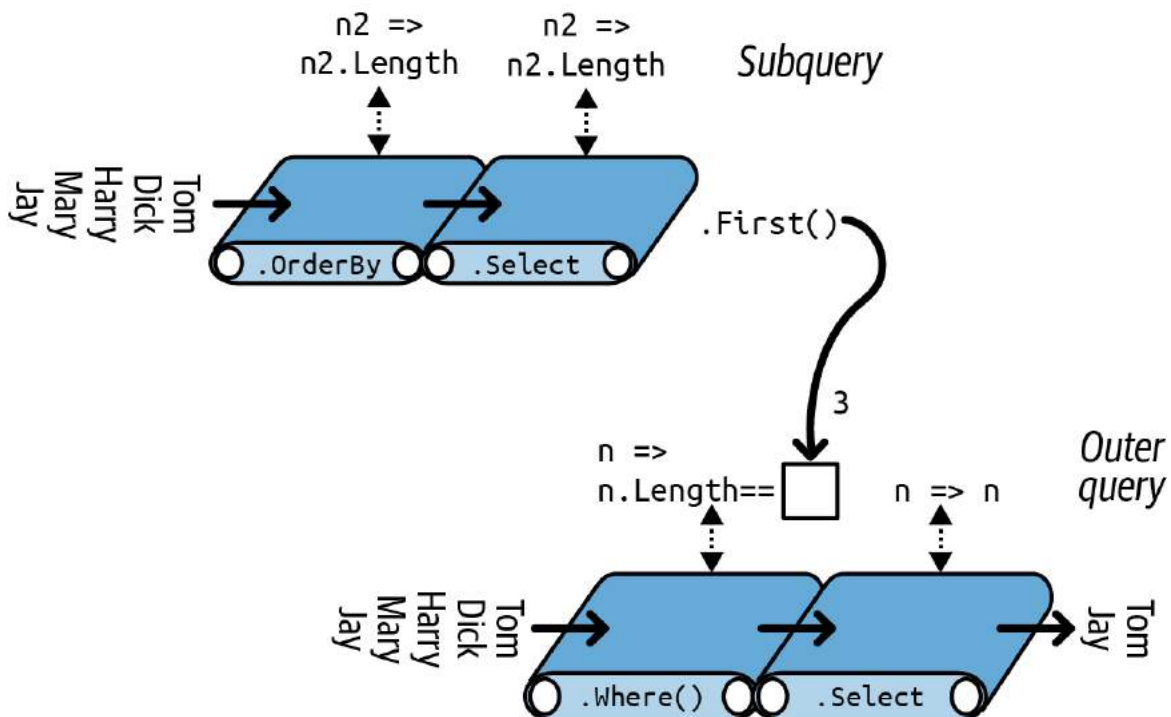
Figure 8-7. Subquery composition
