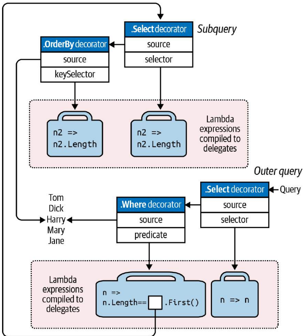
Figure 8-8. UML subquery composition
