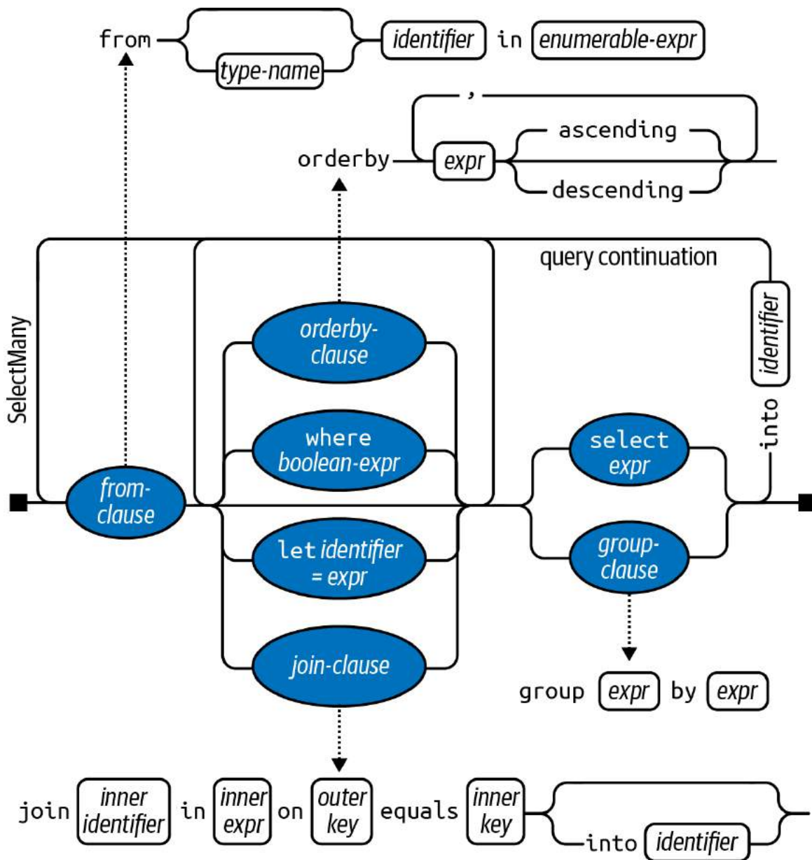
Figure 8-2. Query syntax
